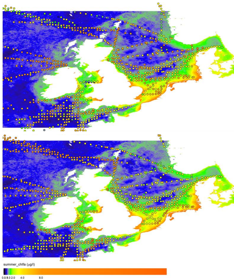
Figure 2.3: Spatial patterns of rescaled season mean diatom abundance over 1960-2019 (circles) in spring (upper panel) and summer (lower panel) in comparison with spatial patterns of growing season mean chlorophyll-a concentrations for 2015 – 2020 based on satellite data by RBINS (background colour).
