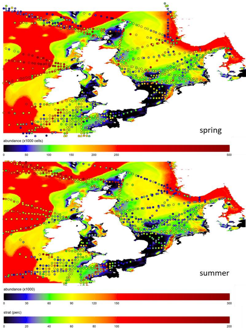
Figure 2.2: Spatial patterns in season mean diatom abundance (circles) in spring in CPR data for 19060 - 2019 (upper panel) and summer (lower panel) overlayed with spatial patterns in percentage of year stratified in model data (background colour).
